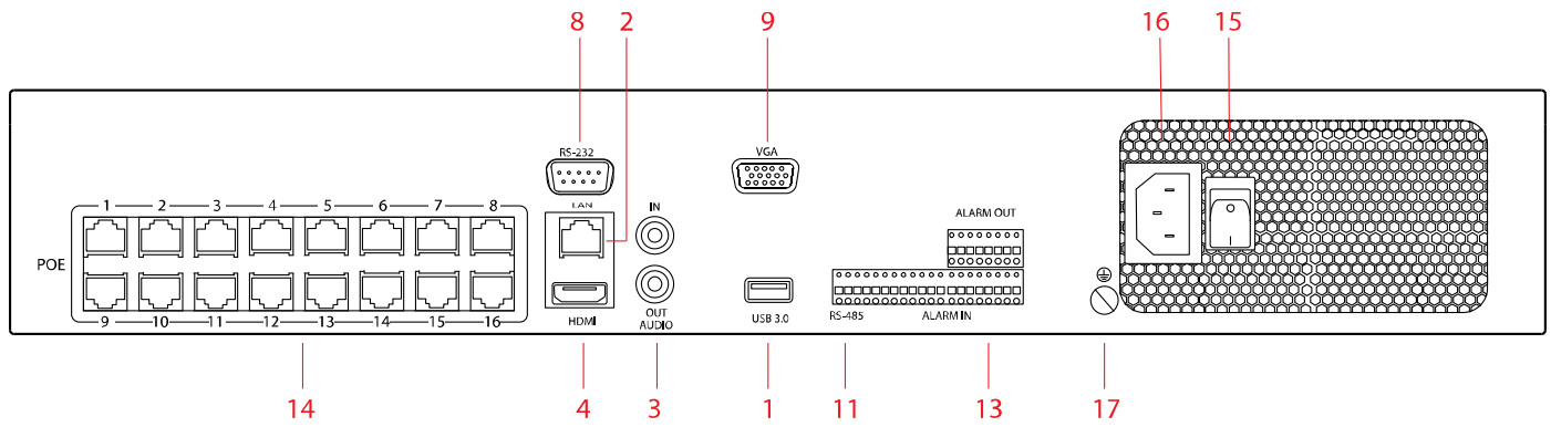
Figure 1, DS-7732NI-I4/16P
