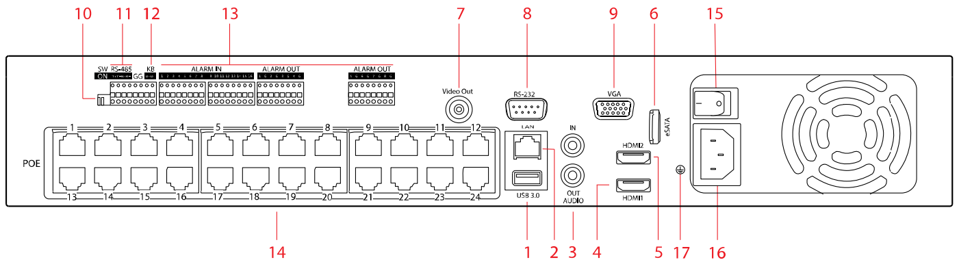
Figure 2, DS-7732NI-I4/24P
